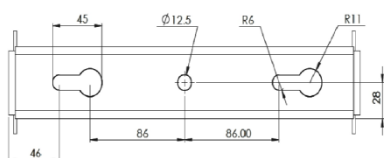
Bracket Top View
